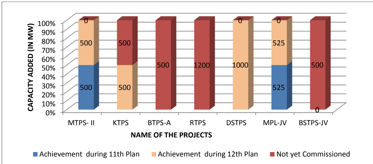
Chart: 2 Status of capacity addition
