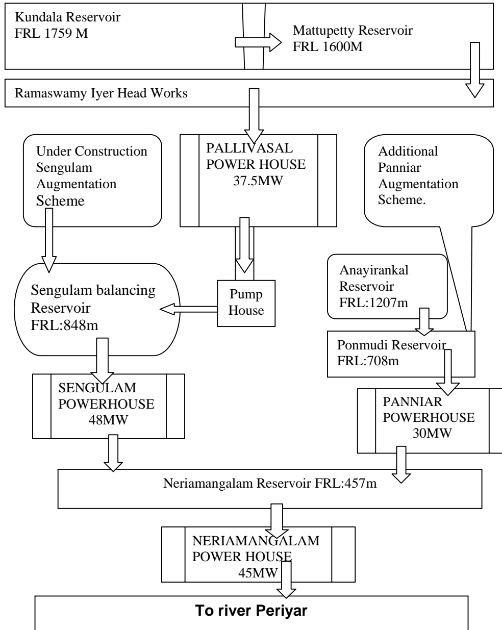
Flow Chart showing the sources of water and generation of power at Pallivasal, Sengulam and Panniar hydro power projects
